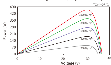
Power-Voltage Curves (48QL6-DB 470W)
