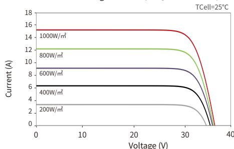
Current-Voltage Curves (48QL6-DB 470W)
